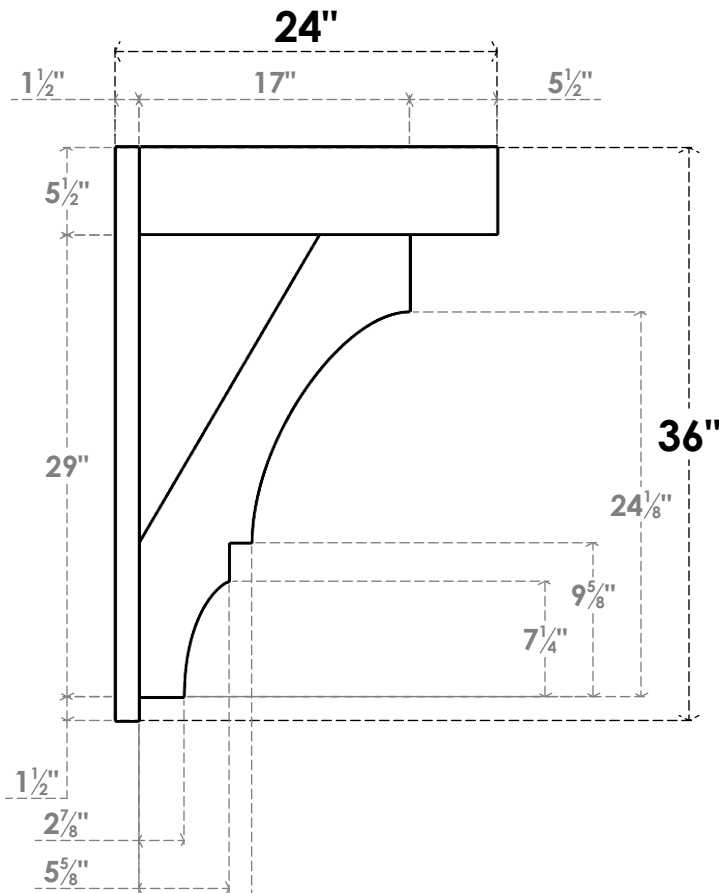
SIDE PROFILE
